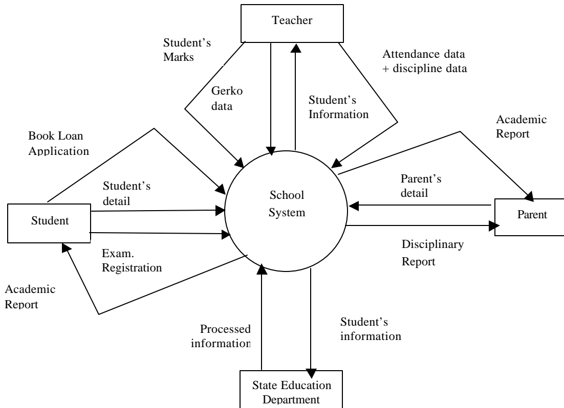
Data Flows between the schools and other organizations
